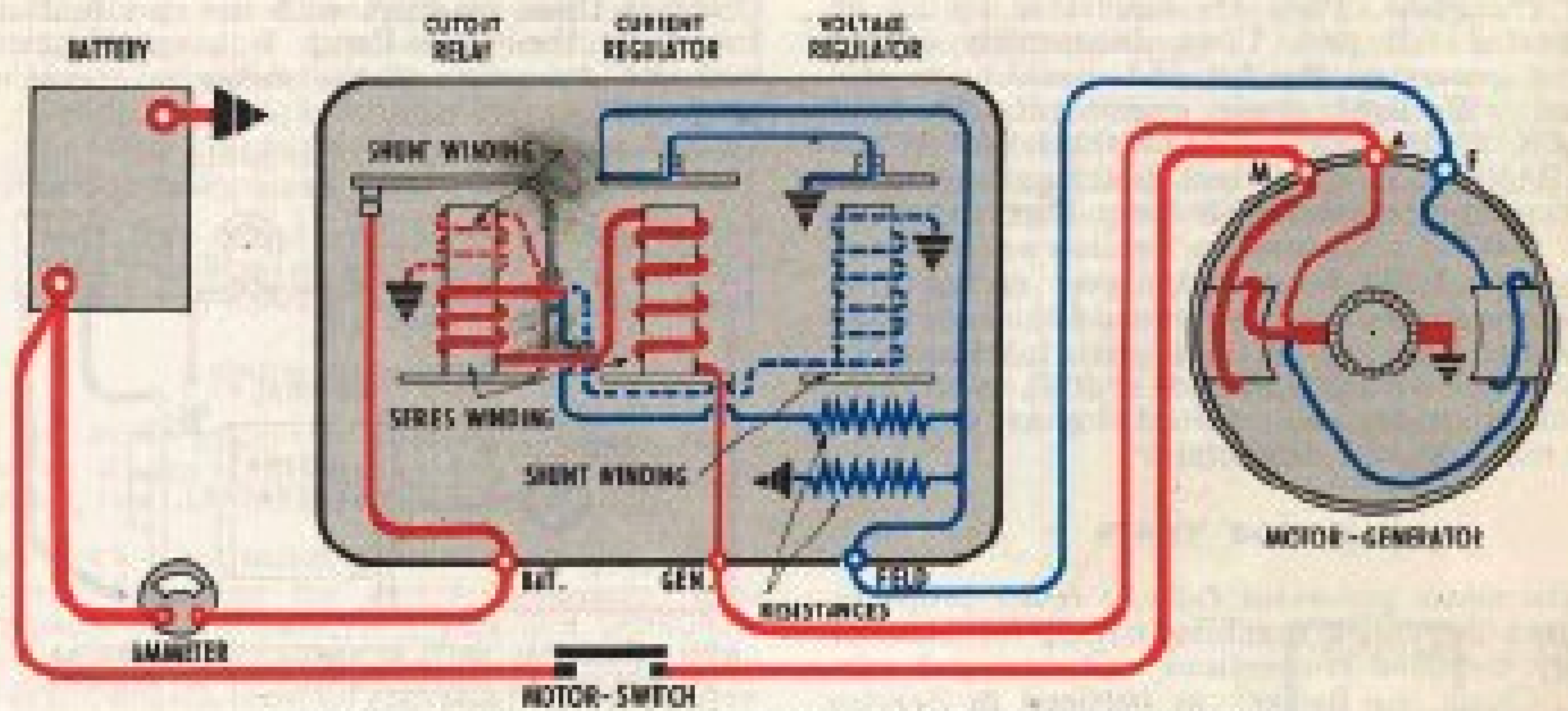
Figure 4—Three terminal motor-generator and three wire regulator wiring.
