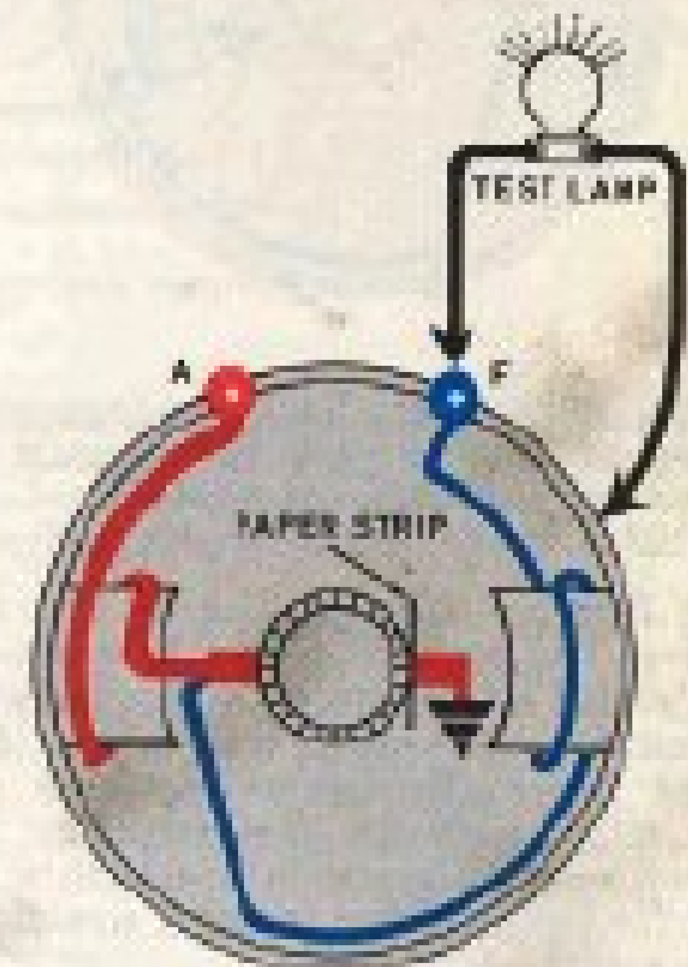
Figure 8—Check for grounded motor-generator.
