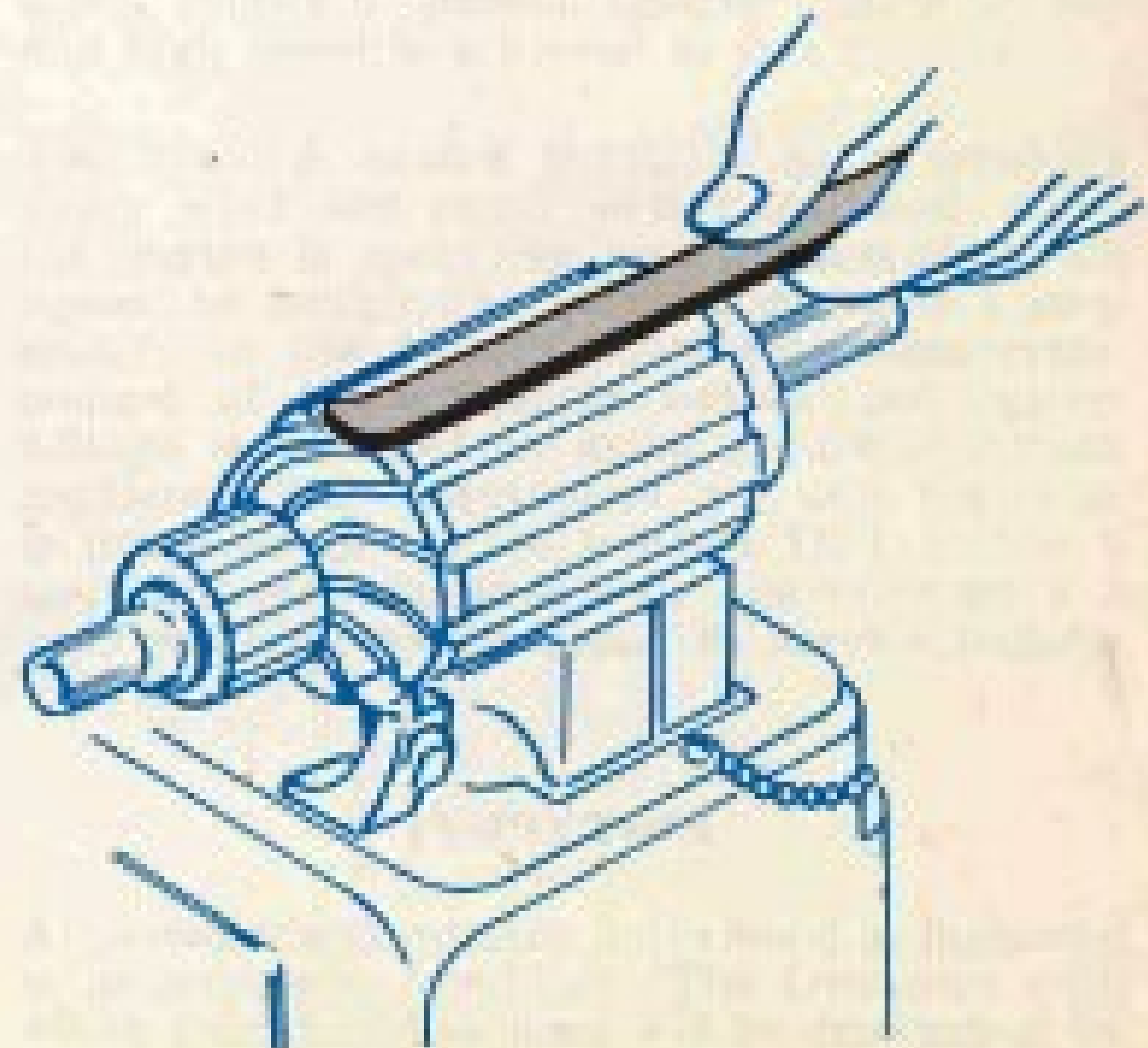
Figure 11—Checking armature for short circuits.
