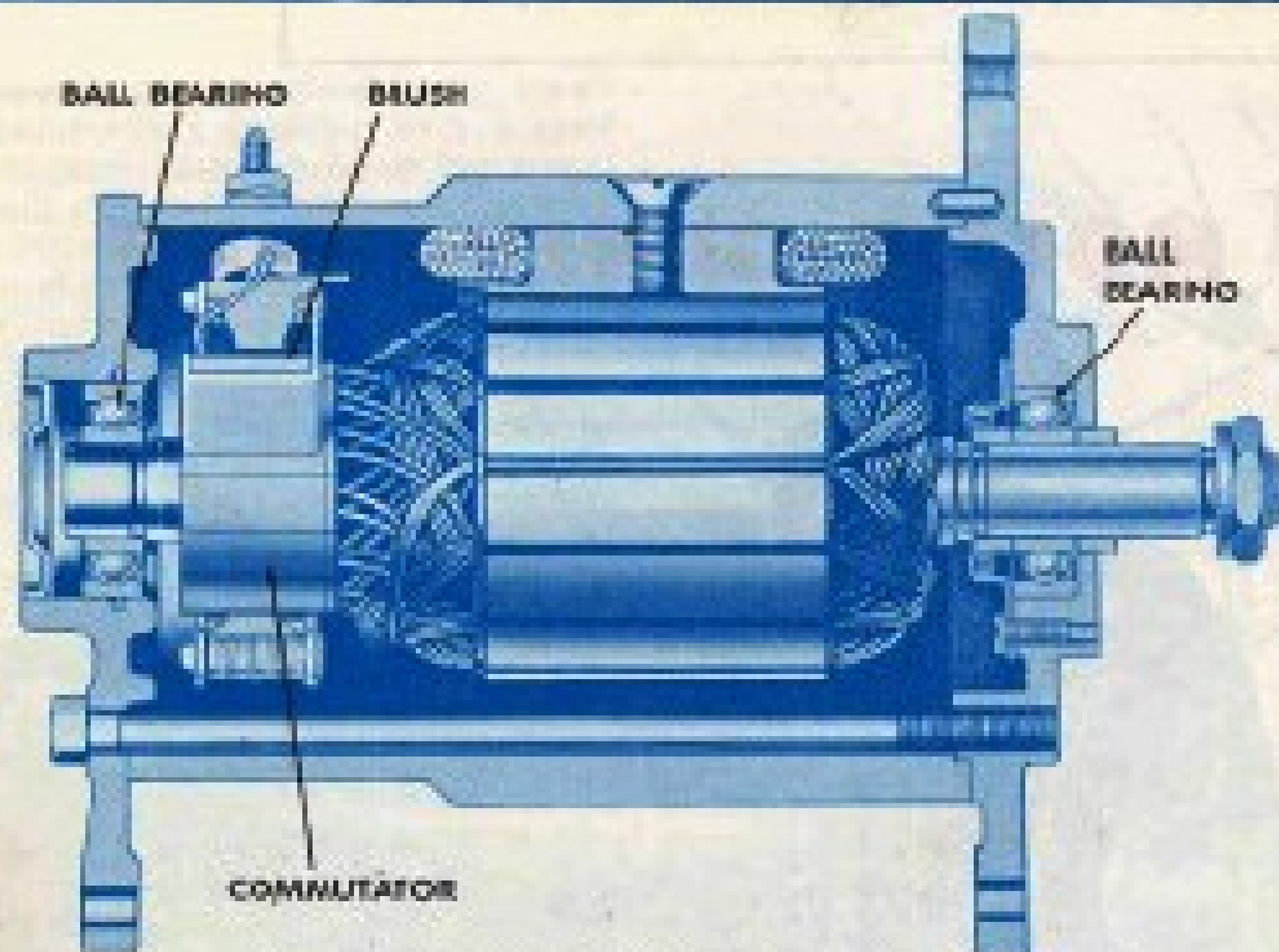
Figure 2—Cross sectional view of motor-generator.
