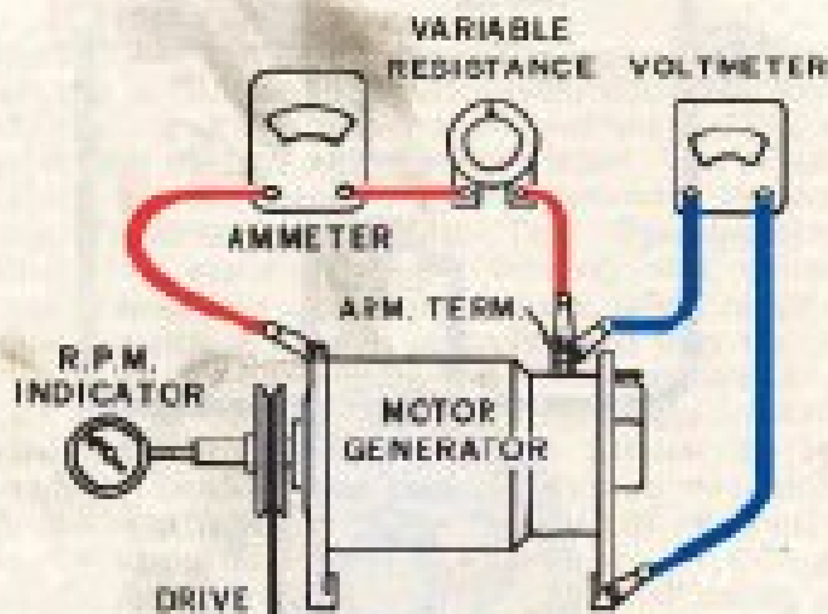
Figure 7—Checking motor-generator output.
